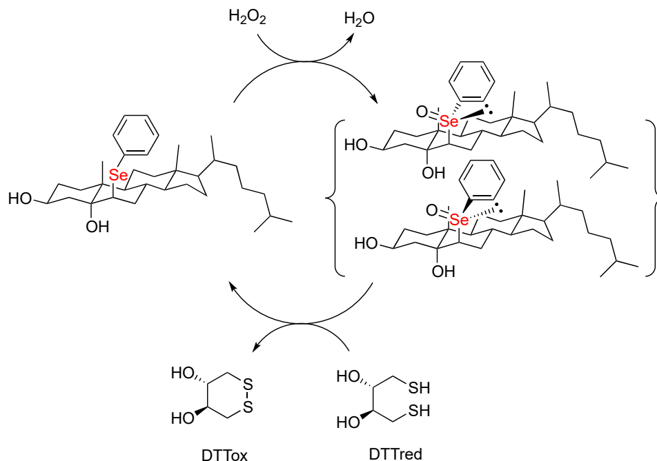
Scheme 3. Proposed redox cycle of 3β,5α-dihydroxy-6β-phenylselenenylcholestane (2).
