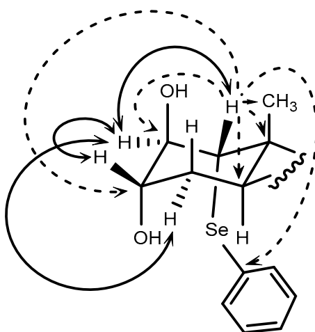
Figure 2. Relevant data from COReletion SpectroscopY (COSY and heteronuclear multiple bond correlation (HMBC) experiments for the structure of the compound 9 (COSY correlations – plain line, HMBC correlations–dashed line, – means no relation).
